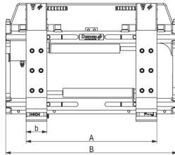
fork positioner for reach truck, no sideshift, bolt-on forks, small frame
