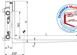
fork positioner for reach truck, no sideshift, bolt-on forks, small frame
