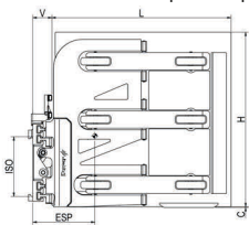
PE = both arms with single articulation
