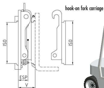
base frame with hook-on fork carriage installed
