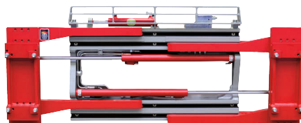
adaptors allow the use of hook-on forks
